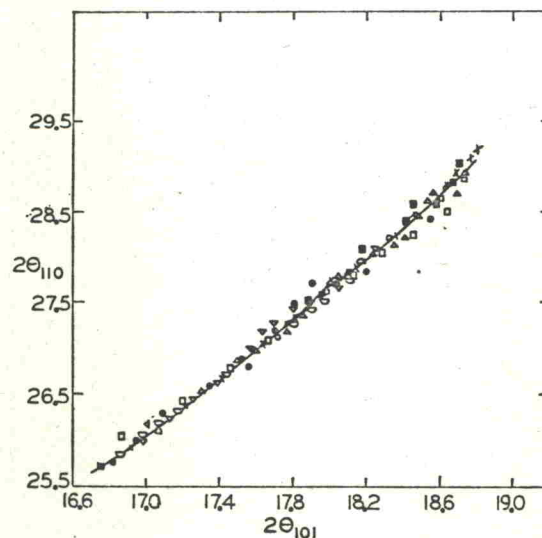
FIG. 2. Diffraction angle 2\theta_{110} versus 2\theta_{101} —magnesium.
